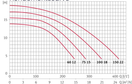
Rendementscurve
